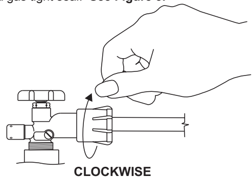
CLOCKWISE Figure 3
