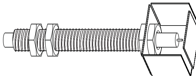
COLLECTOR BOX ASSEMBLY R3B ONLY
