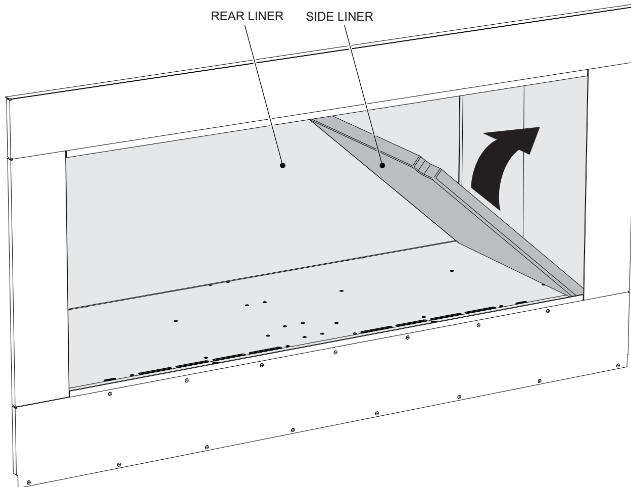
Install Side Liner Figure 49
