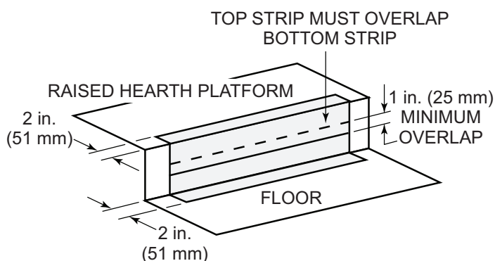
Protect The Front Of A Raised Platform Figure 11
