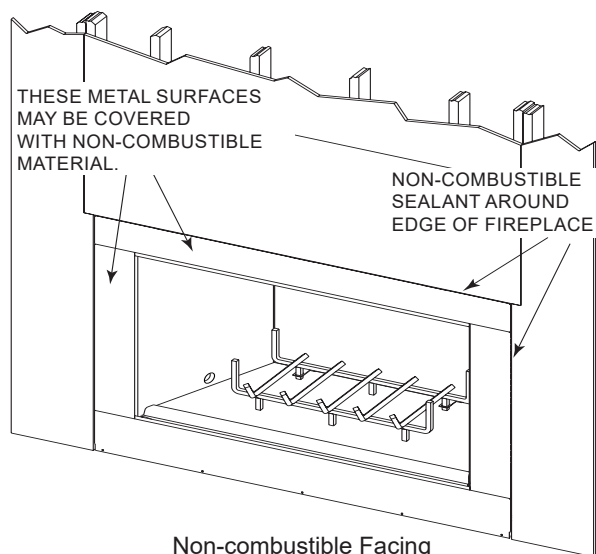
Non-combustible Facing Figure 34
