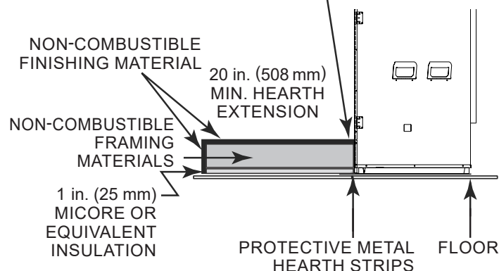
Raised Platform Hearth Extension Detail Figure 38
