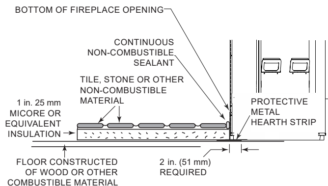
Hearth Extension Construction Figure 37
