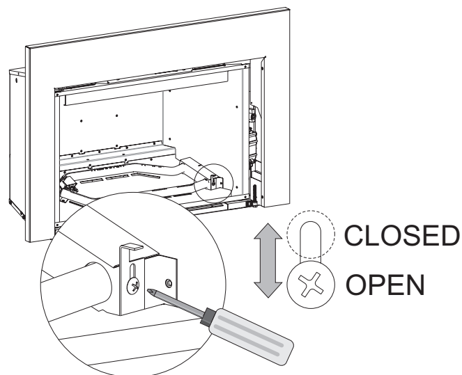
Front Air Shutter Adjustment Figure 21
