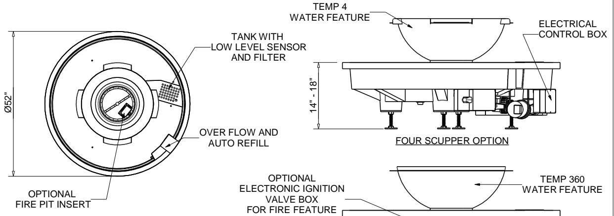
WATER PIT WITH OPTIONAL FIRE PIT
