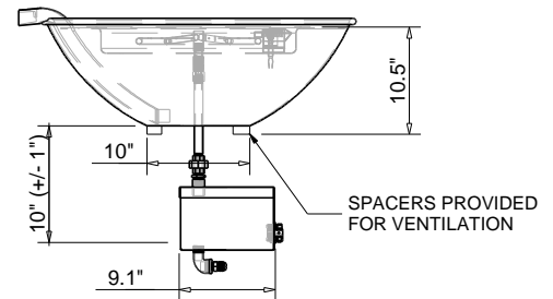
ELECTRONIC IGNITION OPTION
