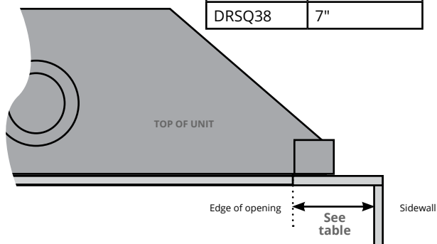
Figure 17.b Sidewall clearances
