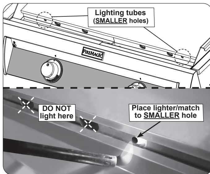
Fig. 37-3 Manual lighting
