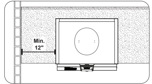
Fig. 19-2 Side wall clearance
