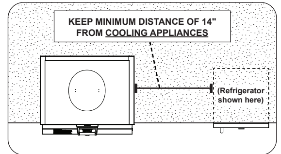
Fig. 19-3 Clearance to cooling appliances
