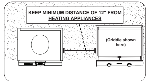
Fig. 19-4 Clearance to heating appliances
