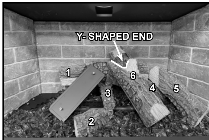
Figure 13 Log #6 Installed
