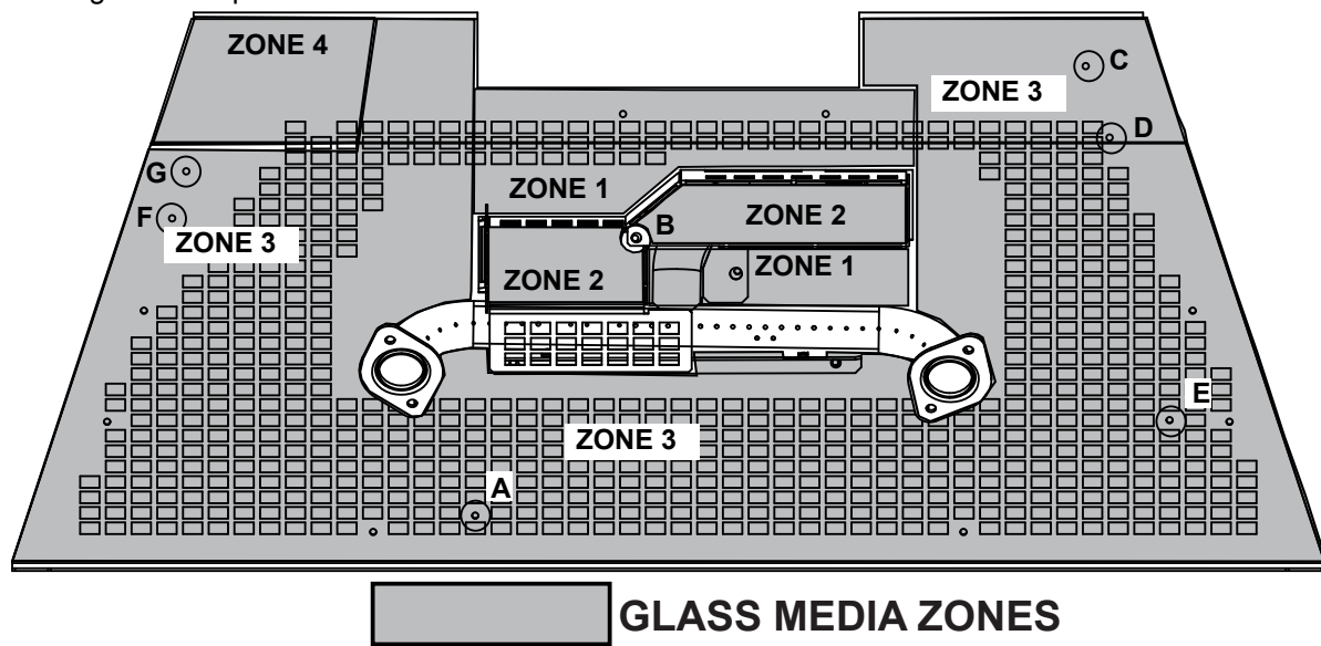
Figure 17 Zone 4 Media Installed
