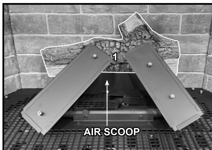
Figure 3 Log #1 Installed
