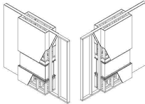
Built-In Bay Installation
