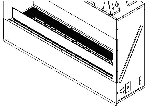
Figure 1. Attach drain pan under appliance
