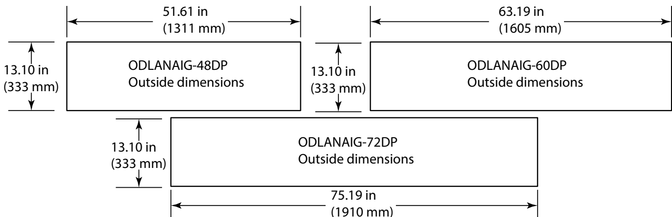
Figure 3. Drain pan dimensions
