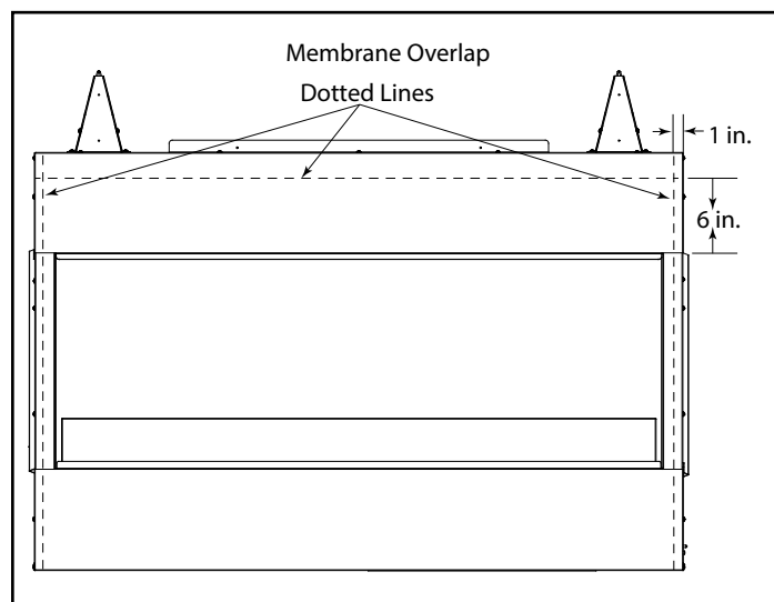
Figure 4.2. Membrane Overlap
