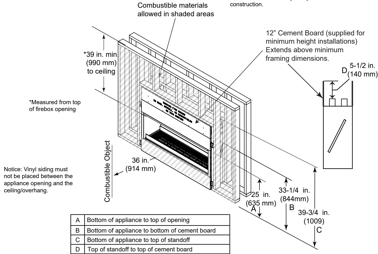
Figure 3.4. Appliance Locations and Framing Dimensions - ODLANAIGST-60
