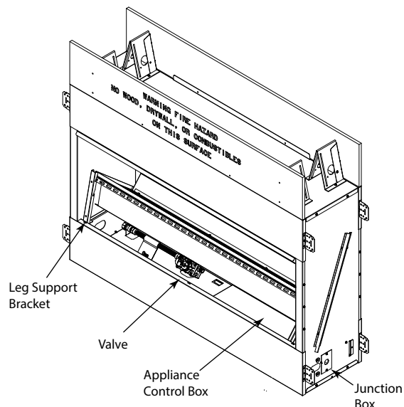
Figure 6.1. Appliance With Engine Lifted
