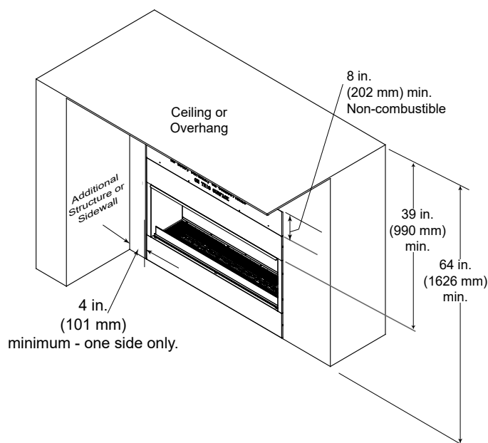
Figure 3.6 Clearances to Combustibles
