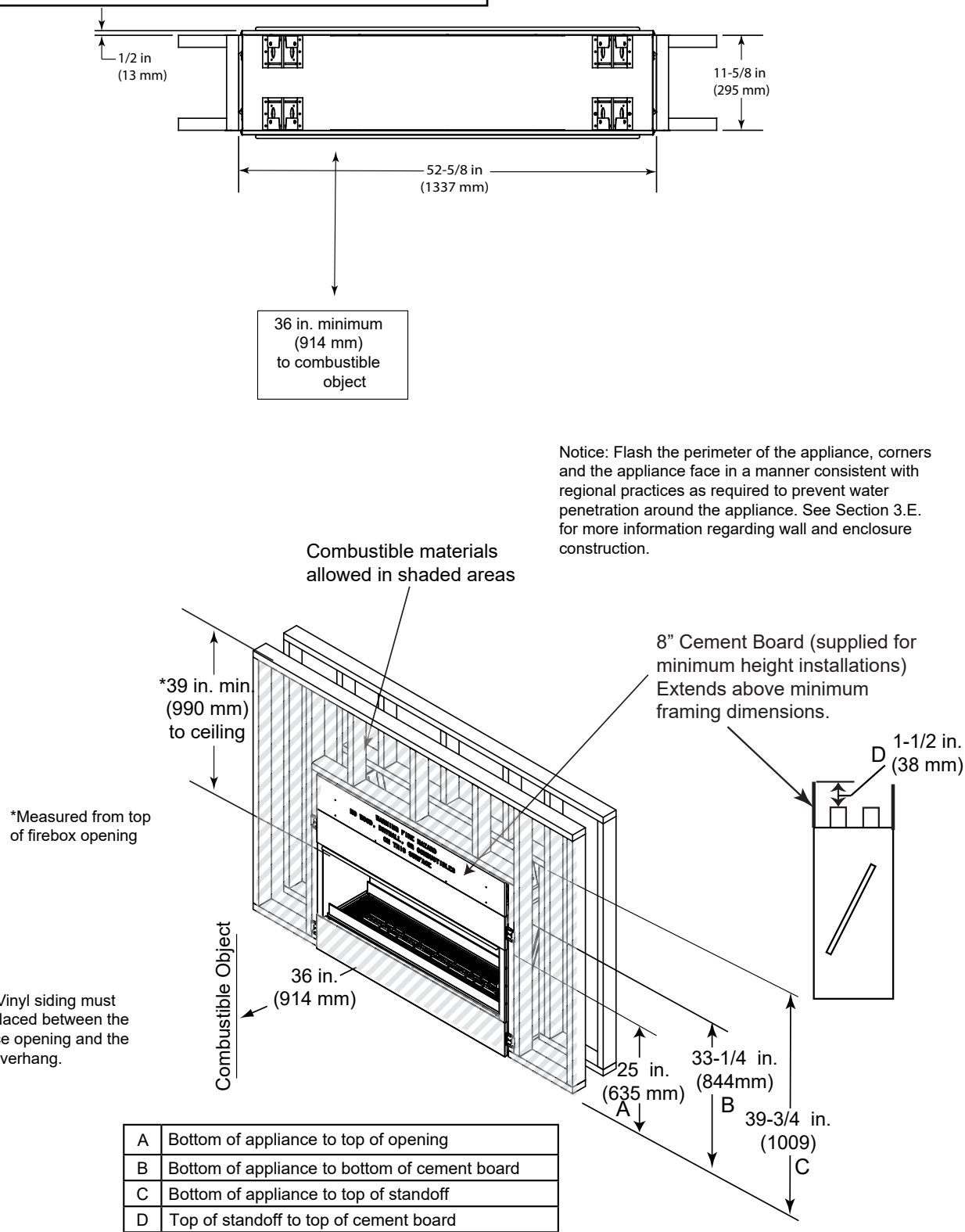
Figure 3.3. Appliance Locations and Framing Dimensions - ODLANAIGST-48
