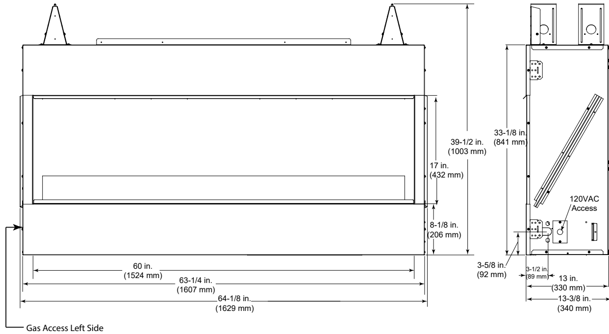
Figure 3.2. Appliance Dimensions – ODLANAIGST-60
