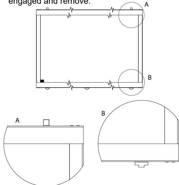
Figure 2. Screen Tabs
