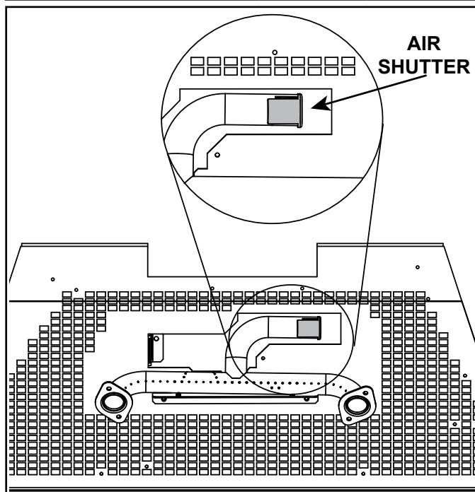
Figure 7.5 Air Shutter
