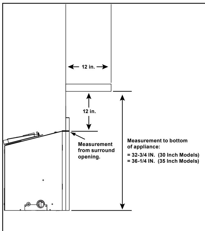
→ Figure 3.15 Minimum Vertical and Maximum Horizontal Dimensions - Combustible
