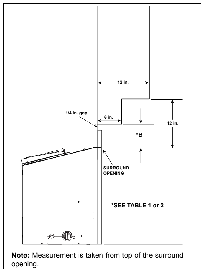
Figure 8.2 Minimum Vertical and Maximum Horizontal Dimensions- Non-Combustible
