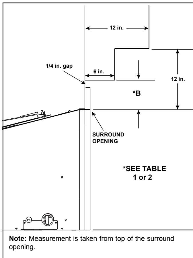
Figure 3.14 Minimum Vertical and Maximum Horizontal Dimensions - Non-Combustible
