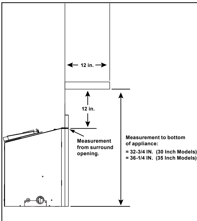
→ Figure 8.3 Minimum Vertical and Maximum Horizontal Dimensions - Combustible
