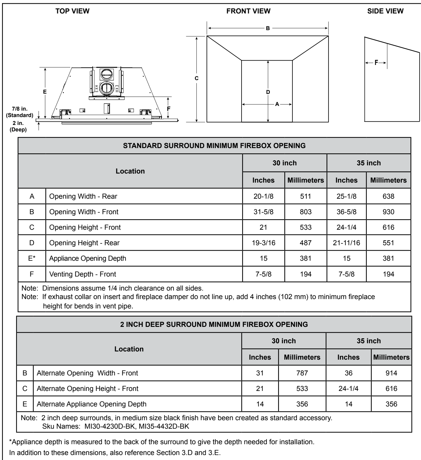
➔ Figure 3.8 Firebox Opening - Standard and Deep Surrounds
