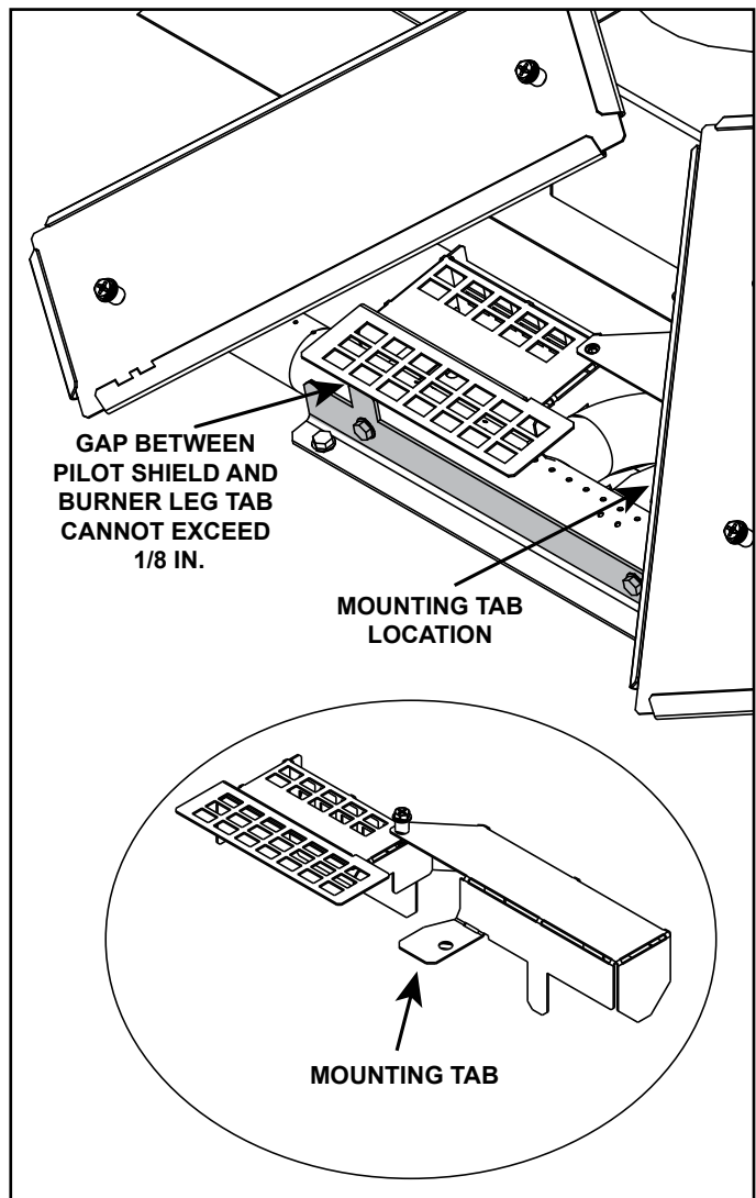
Figure 20 Gap Between Pilot Shield and Burner Leg Tab
