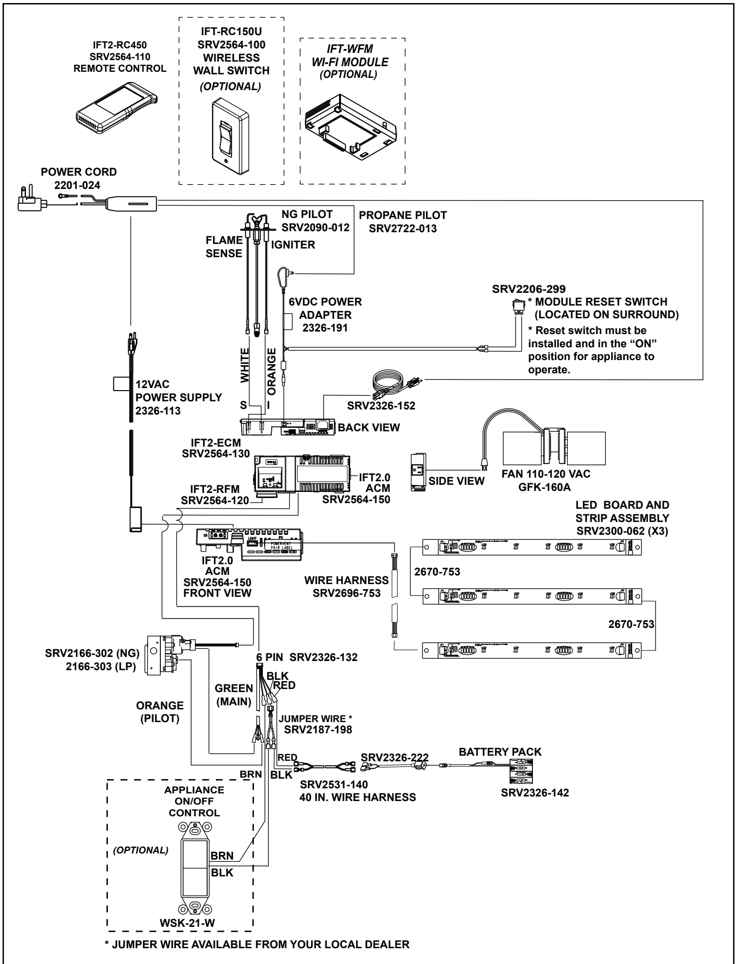
➔ Figure 6.2 IntelliFire Touch 2.0 Wiring Diagram - RUBYP30I
