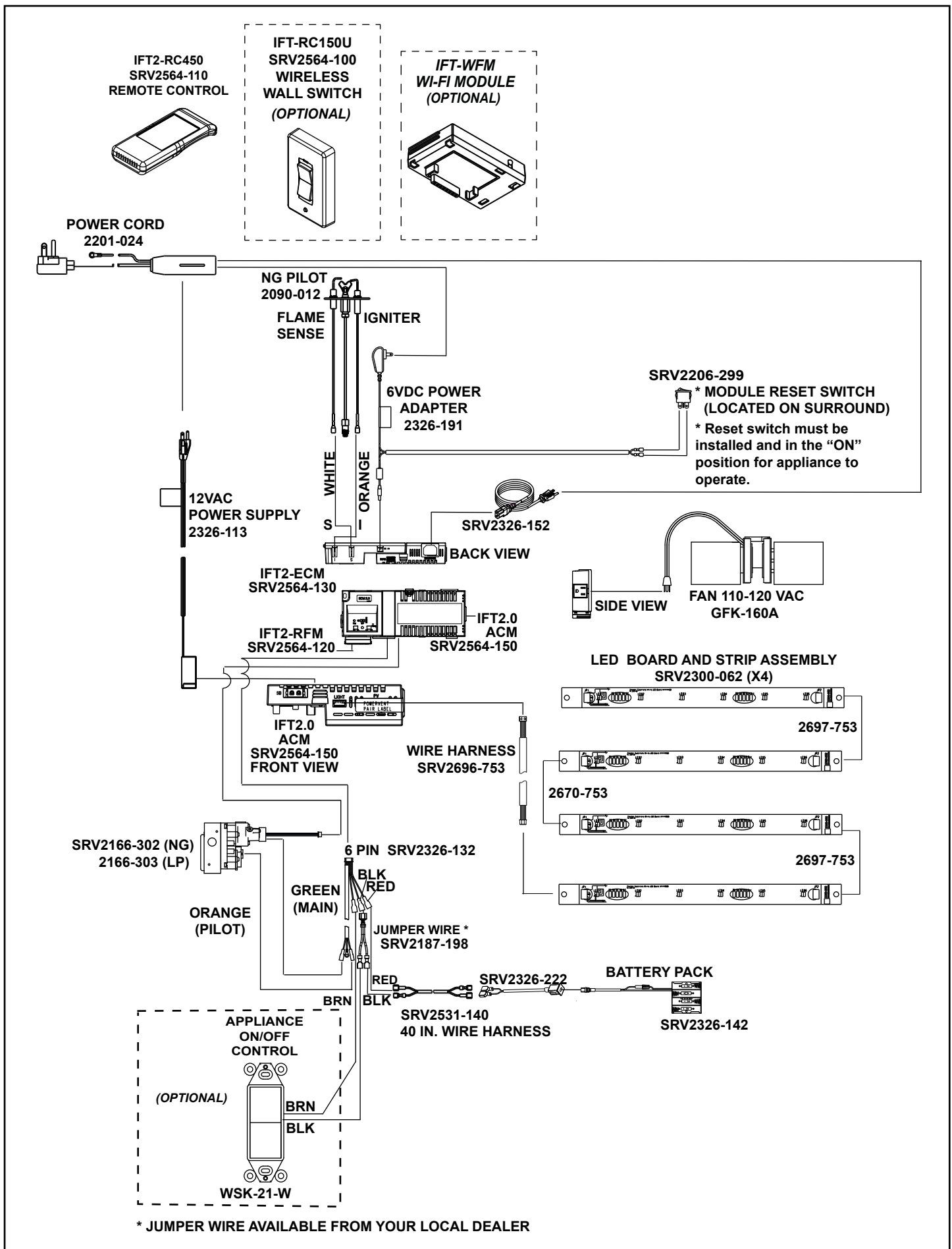
→ Figure 6.3 IntelliFire Touch 2.0 Wiring Diagram - RUBYP35I
