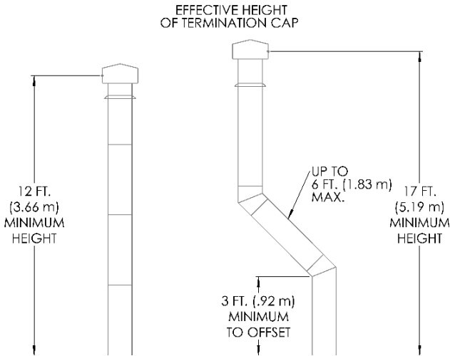
Figure 23 - MINIMUM Vertical Terminations
