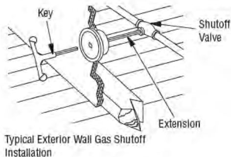
Figure 24 - Manual Shutoff Valve Installation
