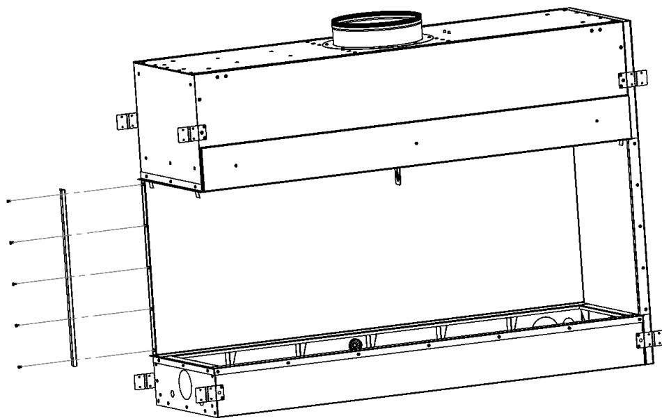
Step 4. Installing left vertical drywall stop.
