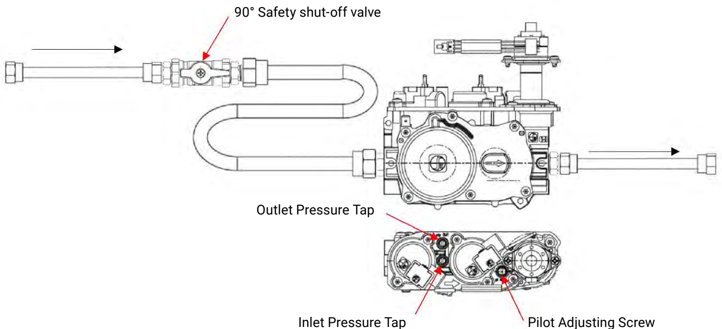
Figure 28 - Connecting Incoming Gas Line to Flex Gas Line
