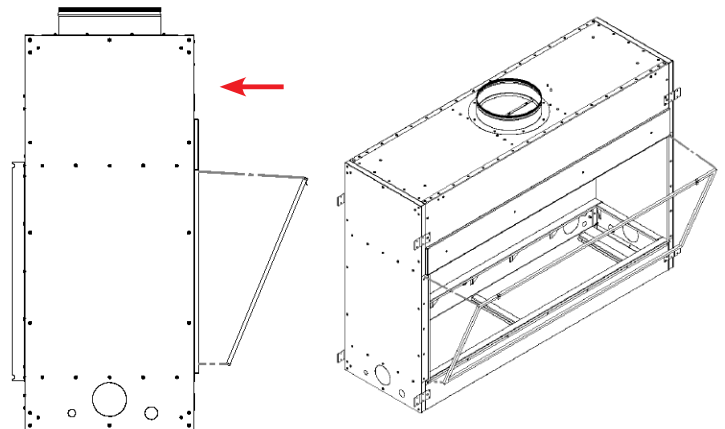
Figure 40 - Invisimesh Installation
