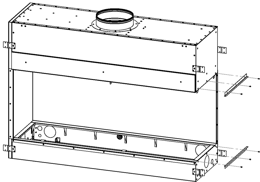
Step 3. Installing right horizontal drywall stops.
