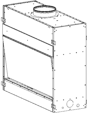
Figure 36 - Rear Panel Installation
