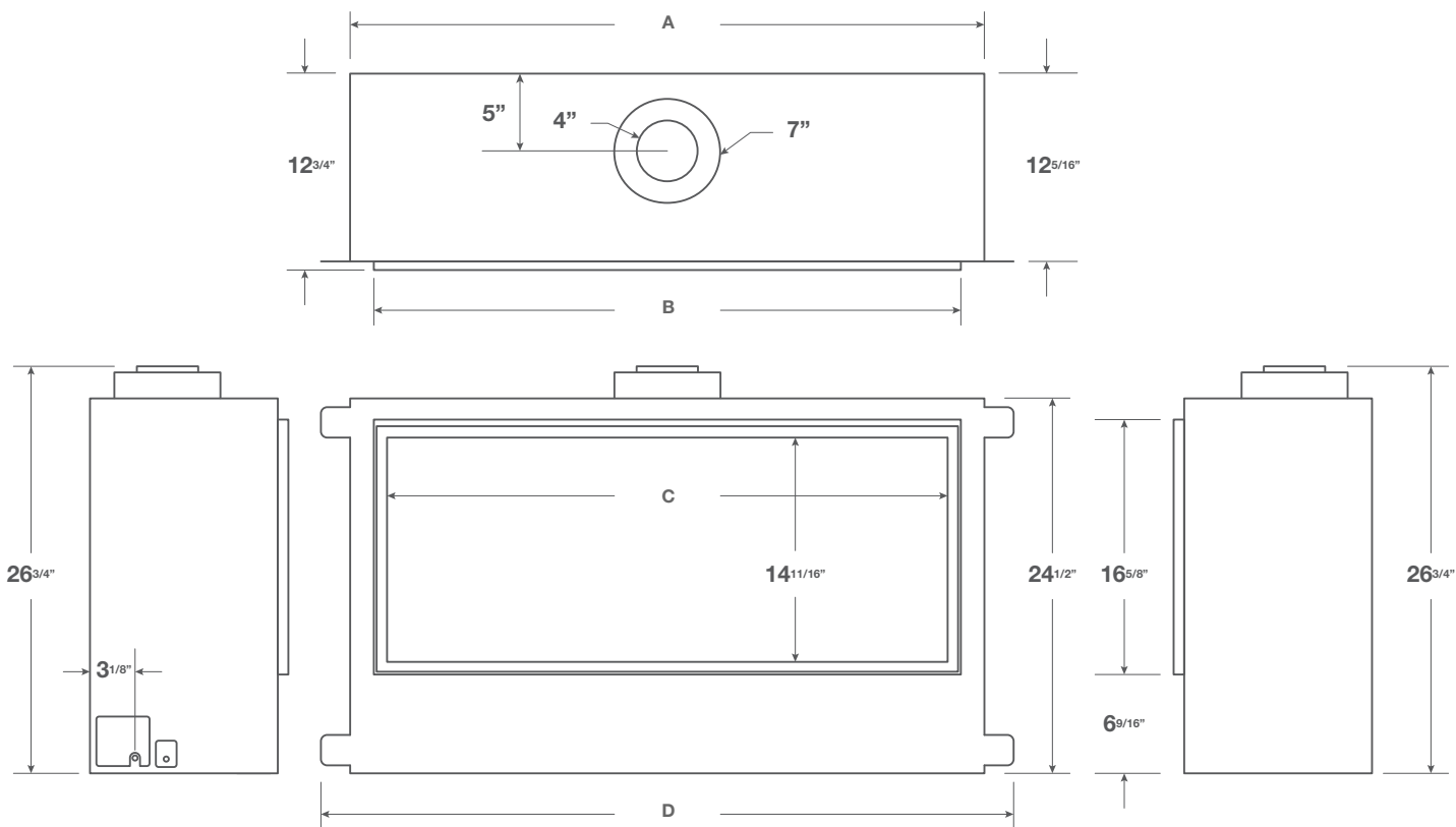
Figure 2. DelRay Fireplace dimensions (Tolerance ± 1/16").
