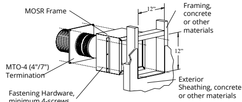
Figure 7.d Installing a MTO termination with MOSR frame.
