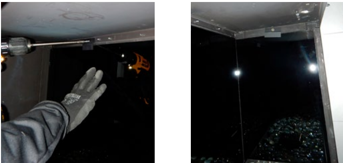
Figure 26.c Secure panel
