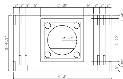
CHIMNEY PLAN
