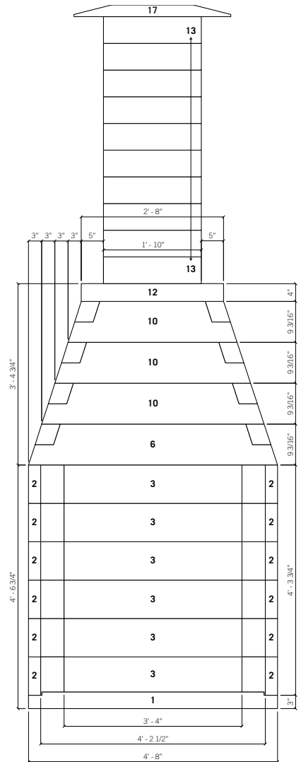
FRONT ELEVATION
