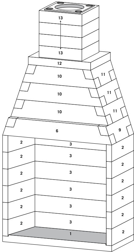
ISOMETRIC
