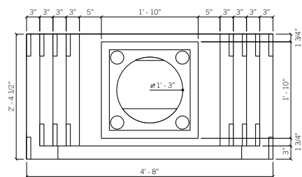
CHIMNEY PLAN
