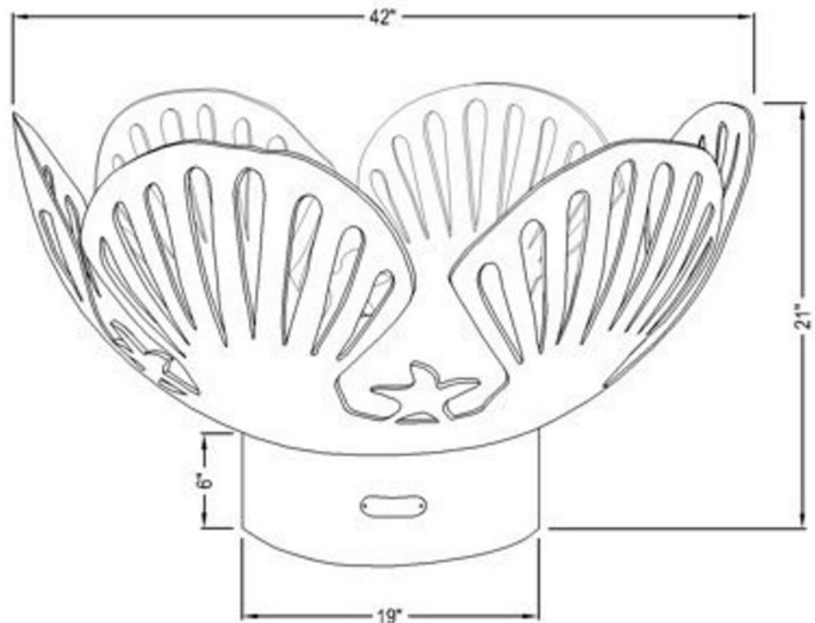
PERSPECTIVE
