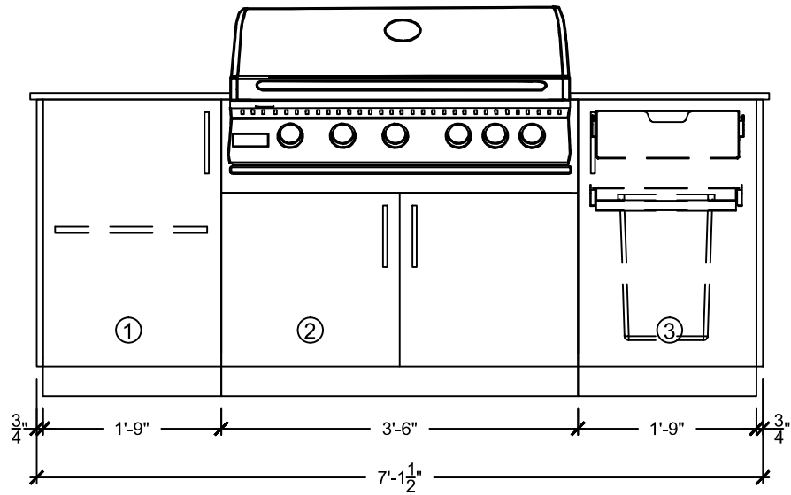
11056 OUTDOOR KITCHEN ELEVATION
