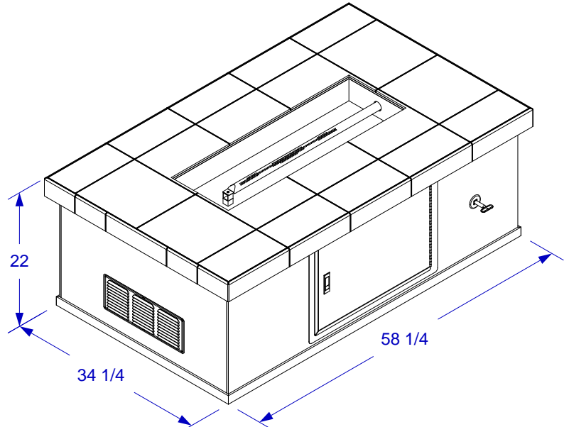
ISOMETRIC VIEW
