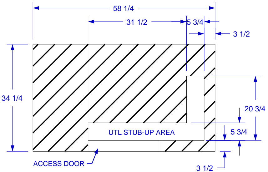
STUB-UP DIAGRAM (SEE NOTE #2)
