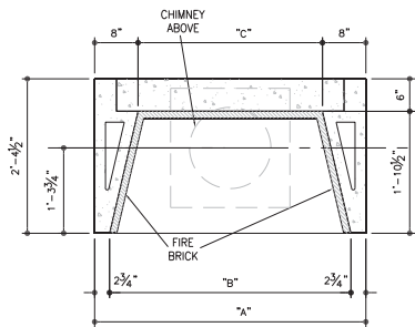
FIREBOX PLAN SCALE: 1" = 1'-0"
