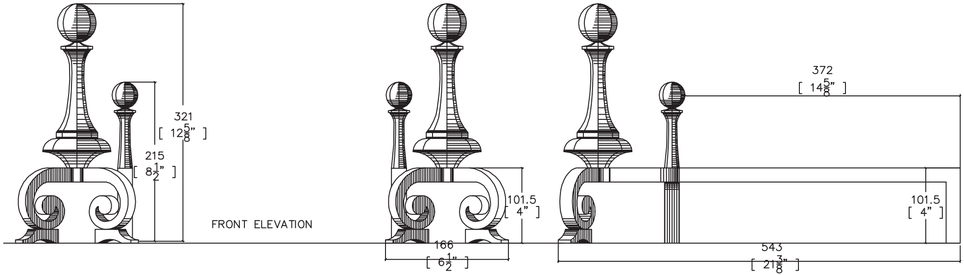
SIDE ELEVATION
