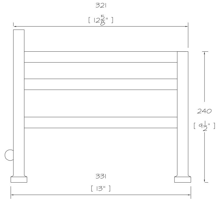
SIDE ELEVATION
