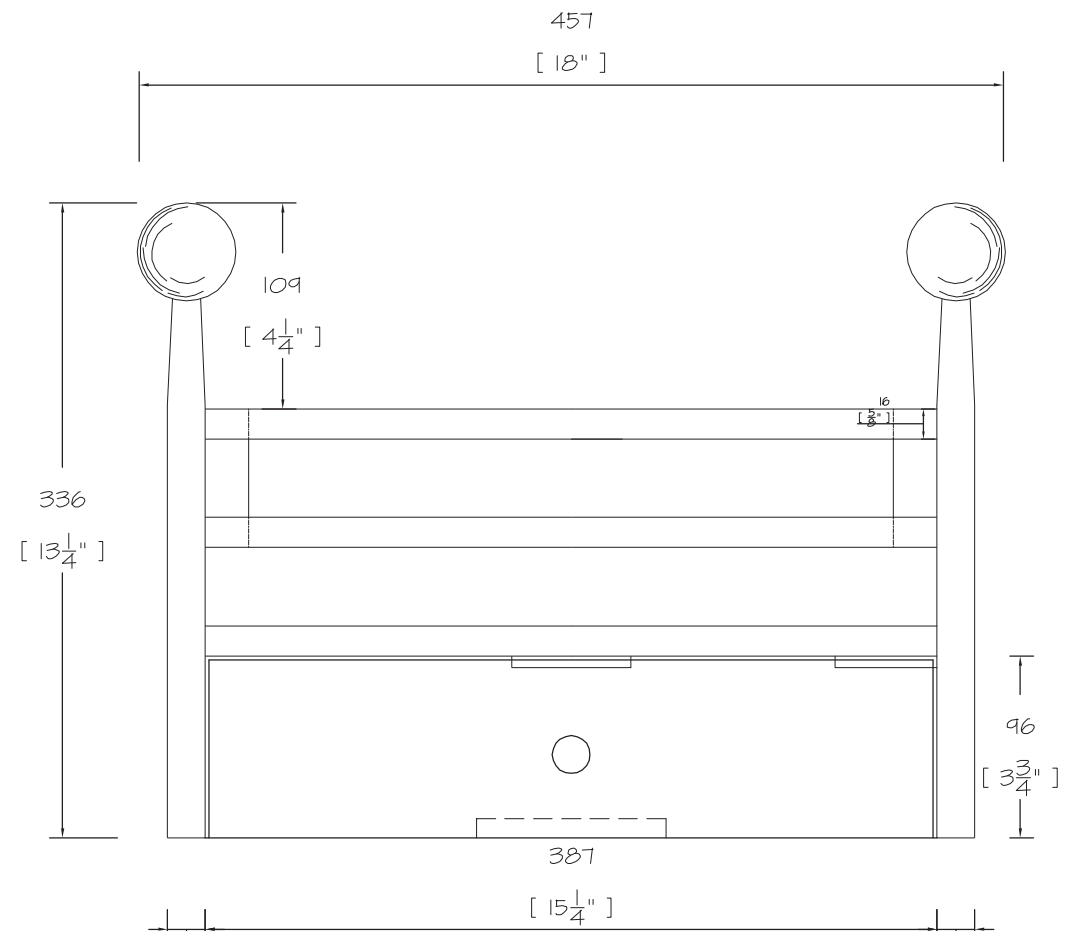
Front Elevation
